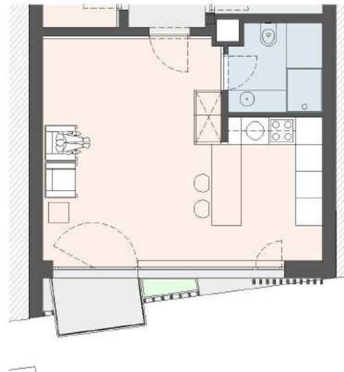
Planta do apartamento Apartment blueprints
